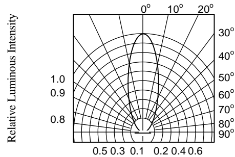
FIG.6 RADIATION DIAGRAM
